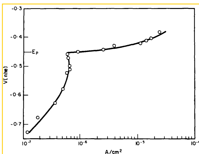
FIG. 2. Anodic polarization curve of 99.99%Al in deaerated 0.1M NaCl solution Ep: potential at which pitting starts.
