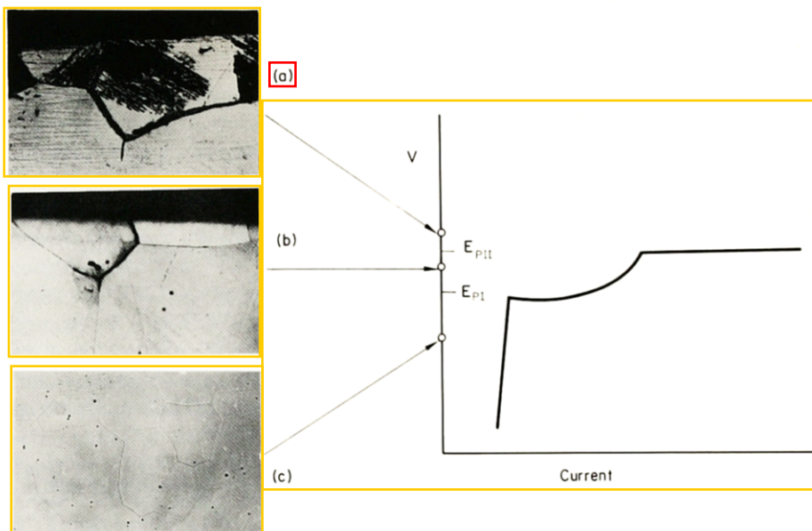
FIG. 7 Anodic polarization curve and type of attack for aged Al-4%Cu in deaerated 1M NaCl solution. Exposure conditions: a = 20 min at -0.35 V(nhe) intergranular corrosion plus tunnel-like pitting, section ( 120\times ); b = 20 min at -0.43 V(nhe), intergranular corrosion, section ( 120\times ); c = 90 min at -0.66 V(nhe) specimen not corroded, normal view ( 30\times ).
