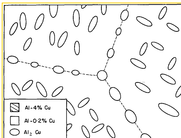
FIG. 10. Schematic representation of the microstructure of over-aged Al-4%Cu alloy Only Al-0.2%Cu and Al_2Cu are present.
